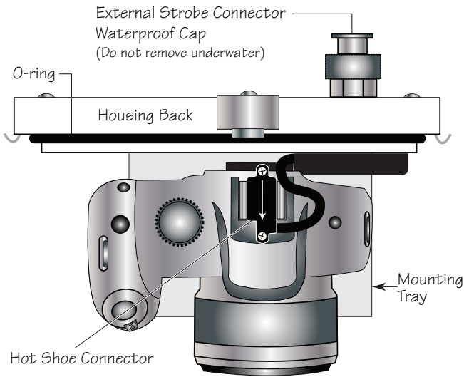
Hotshoe Connector - (SX10IS Shown)
