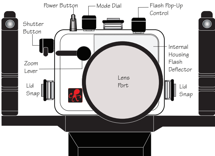
SX1, SX10, SX20 - Front View
